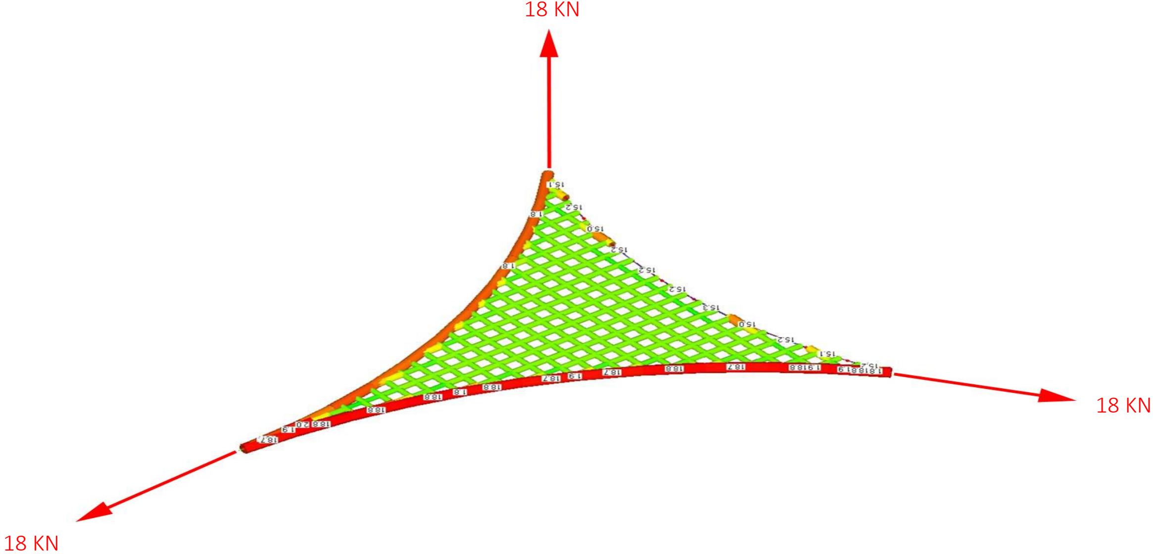
Cable Tension 10 %
